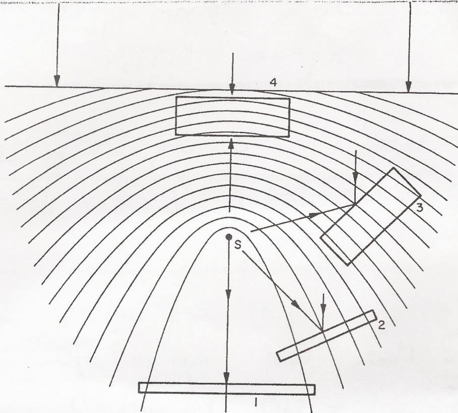
FIG. 1.12. A particular cross section of the family of maximum intensity contour surfaces resulting from interference of a plane wave and a spherical wave originating at S . Representative locations of a hologram plate are indicated.
