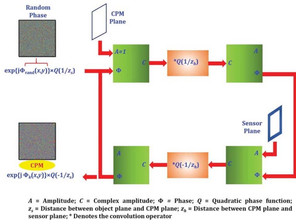
Figure 2. Block diagram of GSA to calculate the CPM.
