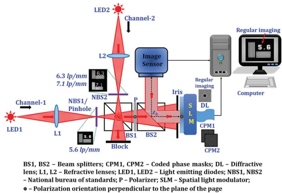
Figure 3. Experimental setup of LI-COACH with two illumination channels.
