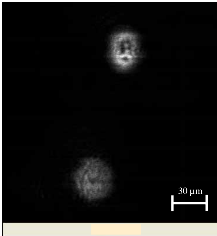
Fig. 3. Movie of the image reconstruction along the light propagation axis.
