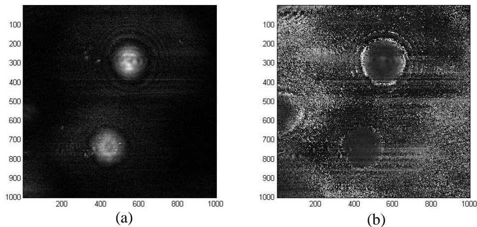
Fig. 3. (a) The magnitude and (b) The phase of the final hologram.
