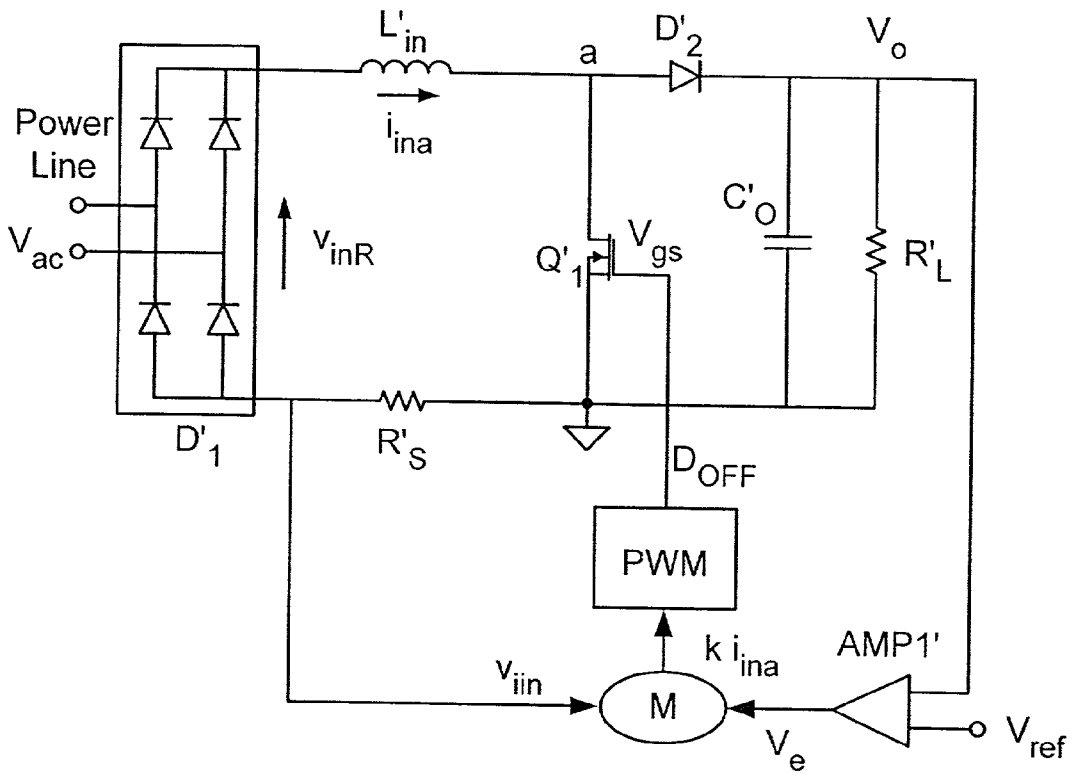
Fig. 3 (Prior art)
