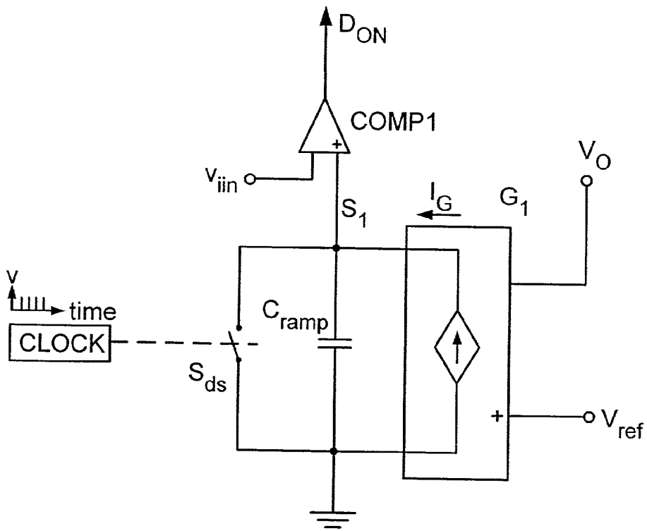
Fig. 4 (Prior art)
