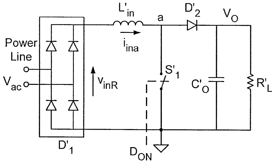
Fig. 1 (Prior art)
