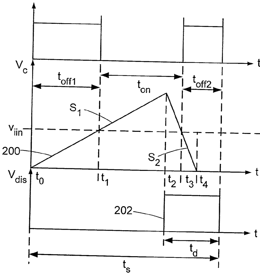
Fig. 6 (Prior art)
