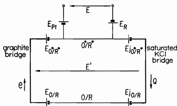
Figure 1. Schematic representation of the cell arrangement proposed by Breck (1972). The half cells E_{O/R} and E_{O^*/R^*} represent the graphite half cells E_{jO/R} and E_{jO^*/R^*} , the liquid junction potentials; E_{Pt} the platinum electrode half cell; and E_R the liquid junction potential of the reference electrode relative to which the platinum electrode is measured.
