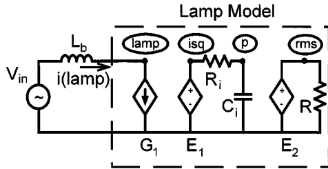
Fig. 3. SPICE-compatible equivalent circuit of a fluorescent lamp.
