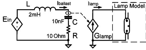
Fig. 11. Separated (tandem) scheme of ballast–lamp system (Fig. 9).
