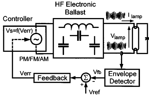
Fig. 2. Electronic ballast for a fluorescent lamp operating in closed loop.
