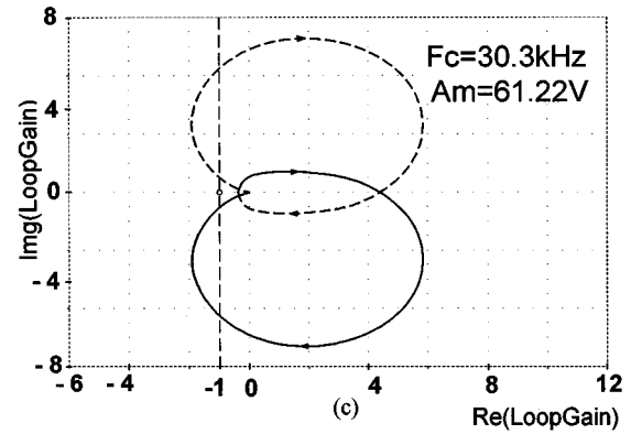
Fig. 13. Nyquist plots of the LoopGain for different values of carrier frequency: (a) F_c = 33.3 kHz (b) F_c = 32.3 kHz. (c) F_c = 30.3 kHz.
