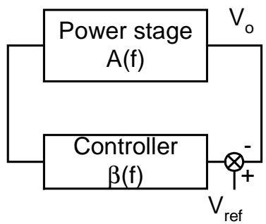
Fig. 4. Basic feedback loop in switch mode converters.
