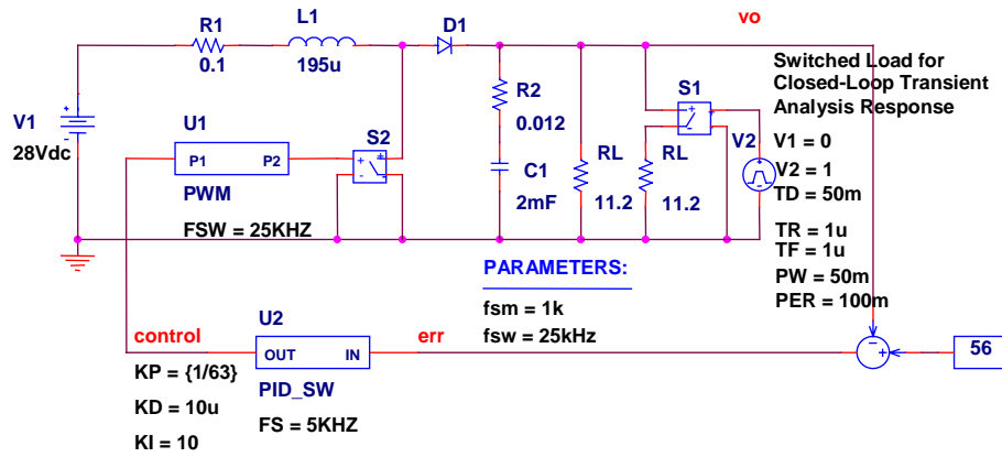
Fig 8. Schematics (PSPICE compatible) of a switched Boost converter [2] with digital PID control (including sample and hold). Sampling period T_s=1/F_s=200\mu S .
