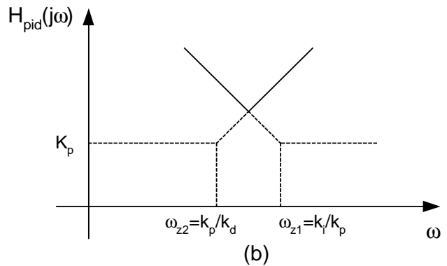
Fig 6. Bode diagrams of PID controller. (a) For \omega_{z1} < \omega_{z2} . (b) For \omega_{z2} < \omega_{z1} .
