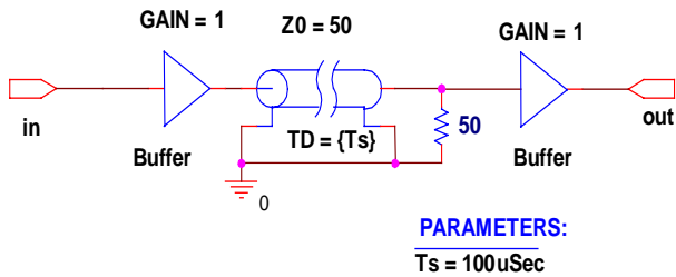
Fig. 1. Continuous equivalent circuit of a pure discrete delay.
