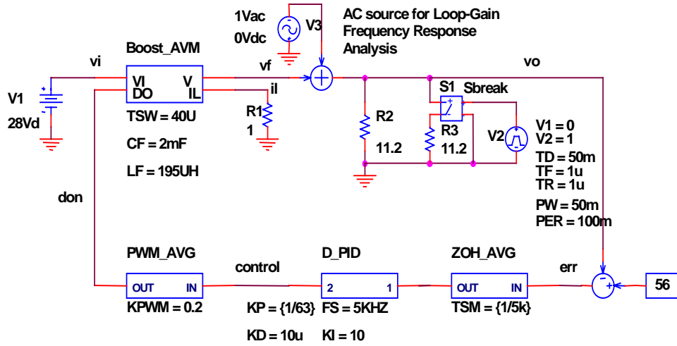
Fig 10. Behavioral model of the digitally controlled Boost converter shown in Fig.8.
