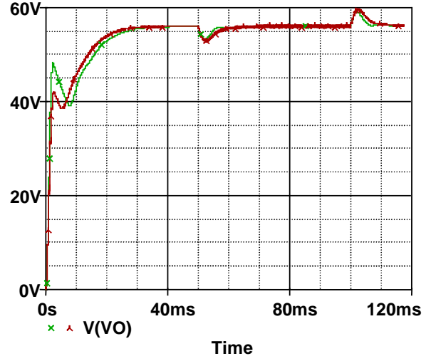
Fig. 13. Time-domain dynamic response of switched (stars) and averaged (crosses) simulation of the closed loop Boost converter.
