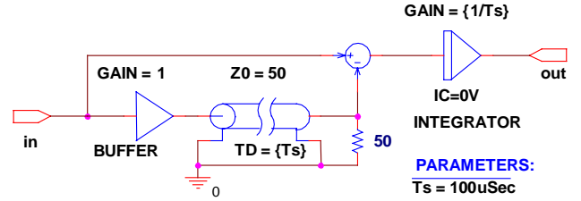
Fig 2. Average model of the ZOH function (ZOH-AVM).
