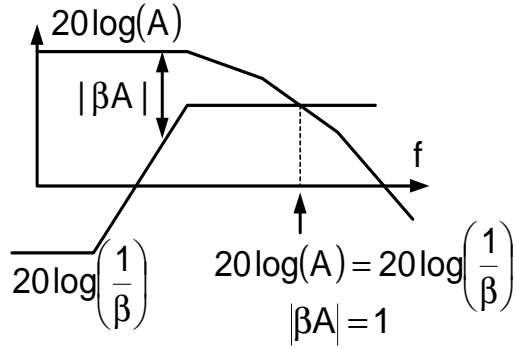
Fig. 5. Bode plot design of loop gain based on a fixed A(f) and adjustable 1/\beta(f)
