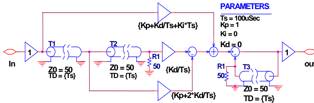
Fig 3. Digital PID Average Model (D_PID_AVM).
