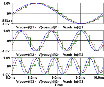
Fig 11. Typical waveforms of ZOH-AVM as compared to discrete ZOH for three different frequencies: 500Hz, 1.5kHz and 2.5kHz. Input voltage: continuous, leading. Output of discrete ZOH: stepped. Output of ZOH-AVM: continuous, lagging.
