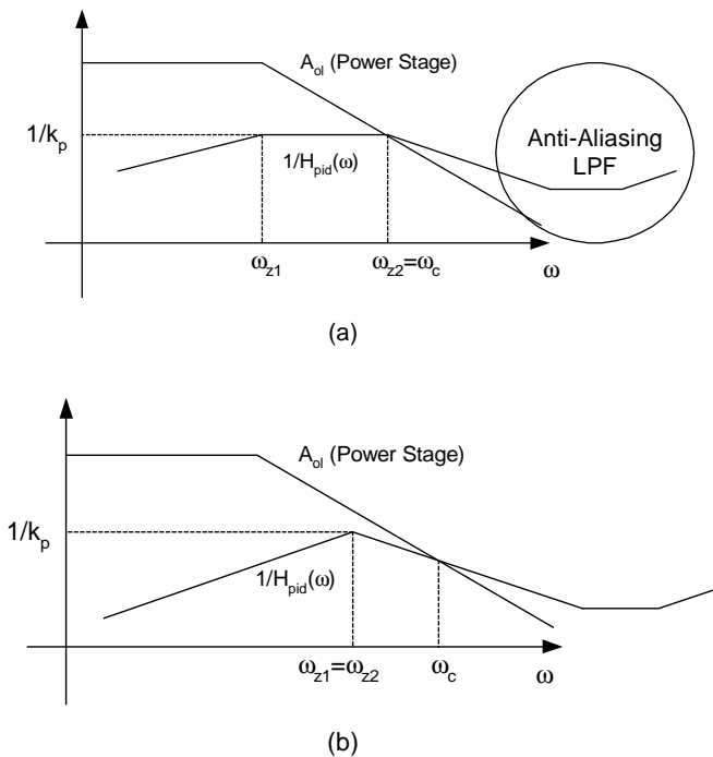
Fig 7. Suggested design steps for the digital PID. (a) Starting point. (b) Final (optimized) point.
