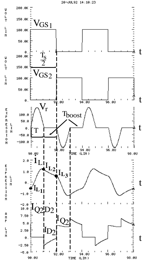
Fig.3. Expected waveforms of proposed CS-PPRI. (simulated by HSPICE, MetaSoftware Co.)
