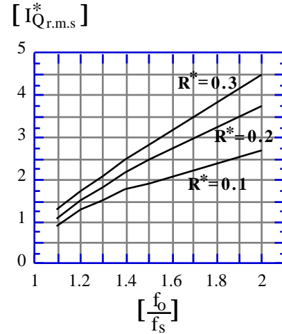
Fig. 7. Normalized transistor current ( I_{Qr.m.s}^* ) as a function of the normalized switching frequency ( f_0/f_s ) with the normalized load ( R^* ) as a parameter.
