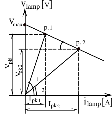
Fig. 13. The proposed model (16) of the V-I characteristic of a fluorescent lamp, when driven by a high frequency sinusoidal current source. See text for details.
