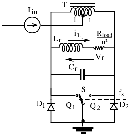
Fig. 2. Simplified equivalent circuit of the proposed CS-PPRI.
