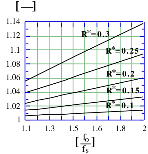
Fig. 4. The normalized quasi-resonant period ( T = 2f_r T ) as a function of the normalized switching frequency ( f_o/f_s ) with the normalized load ( R^* ) as a parameter.
