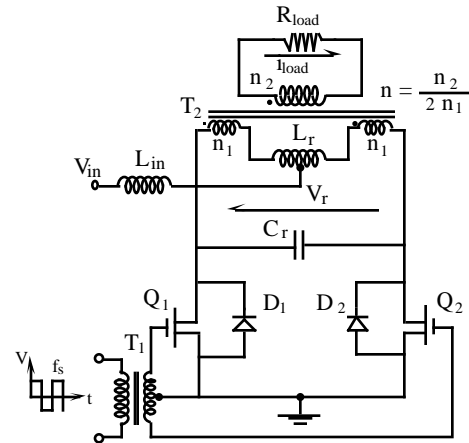
Fig. 1. The proposed Current Sourcing Push-Pull Parallel Resonance Inverter (CS-PPRI).
