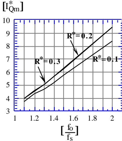
Fig. 5. Normalized transistor current ( I_{Qm}^* ) as a function of the normalized switching frequency ( f_0/f_s ) with the normalized load ( R^* ) as a parameter.
