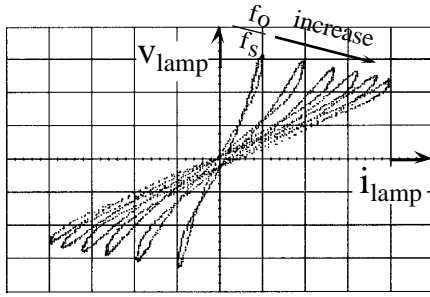
Fig. 12. Measured V-I characteristic of the experimental fluorescent lamp (General Electric type F40D/2) as a function of the frequency ratio f_o/f_s ( f_o/f_s range: 1.1-1.5). Vertical scale: 50 V/div. Horizontal scale: 0.2 A/div. Nominal switching frequency 300 kHz.
