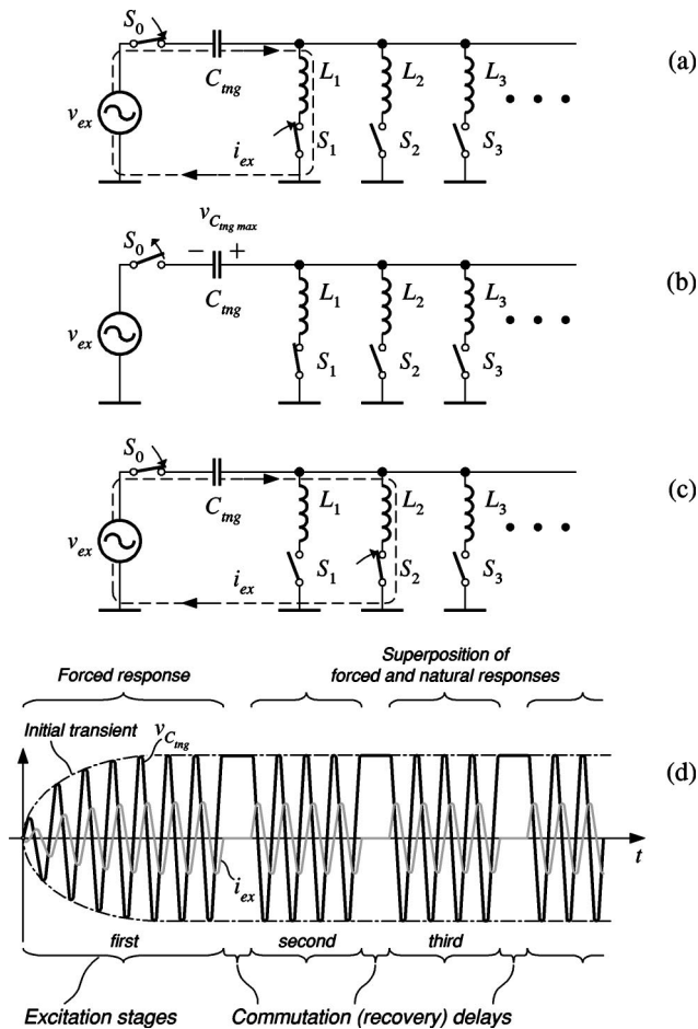
FIG. 2. Commutation method: the commutation of the tuning capacitor and transmitting coils (a) during the first excitation stage, (b) between the excitation stages, and (c) during the second excitation stage, (d) time diagram of the tuning capacitor voltage.
