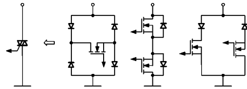
FIG. 4. Replacing the triacs in Fig. 3(a) with faster bidirectional switches can decrease the commutation delays (t'_i, t_{i+1}) in Fig. 3(b).
