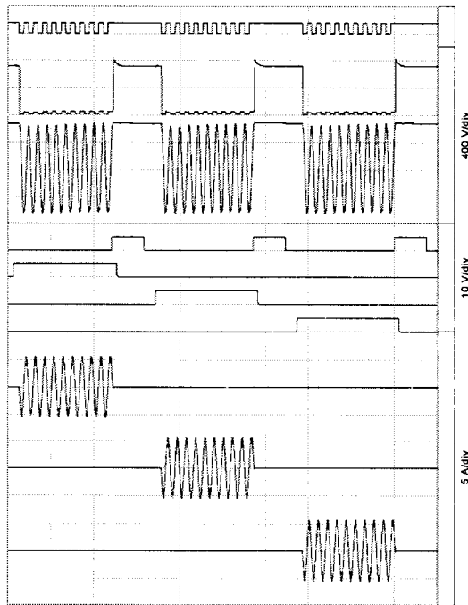
FIG. 3. Implementation of the transient-free commutation method: (a) commutation system and (b) oscillograms.
