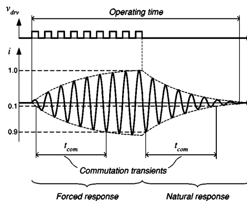
FIG. 1. Conventional commutation of resonant-mode inductors involves long transients.
