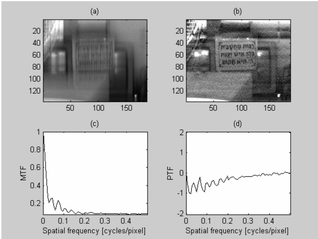
(a) An image is degraded by a mechanical shaker (vertical motion). (b) The restored image using the blind restoration method. (c) and (d) The motion MTF and PTF identified from the image and used for the restoration.
