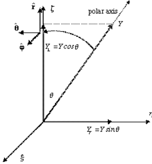
Figure 2. Geometry for spherical coordinates and external magnetic field along the \theta = 0 polar axis.
