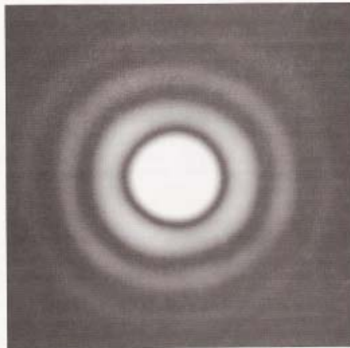
FIGURE 4.10 Fraunhofer diffraction pattern of a circular aperture.
