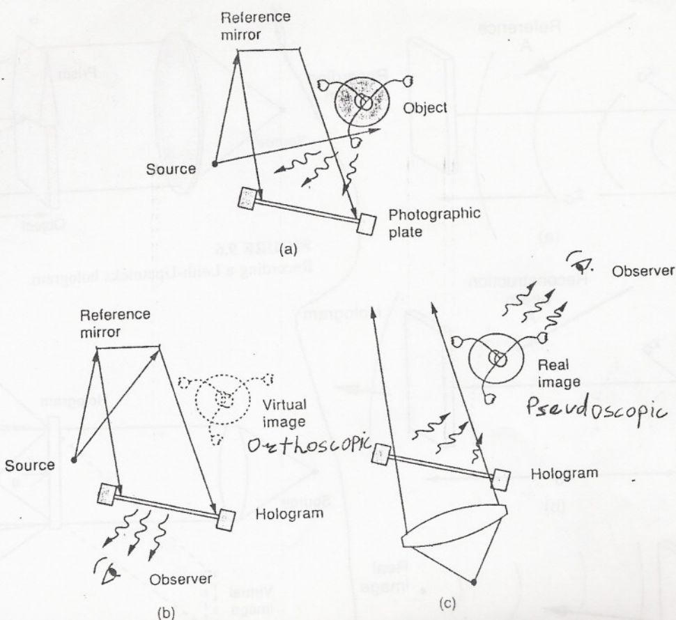
FIGURE 9.9 Holographic imaging of a three-dimensional scene. (a) Recording the hologram; (b) reconstructing the virtual image; (c) reconstructing the real image.
