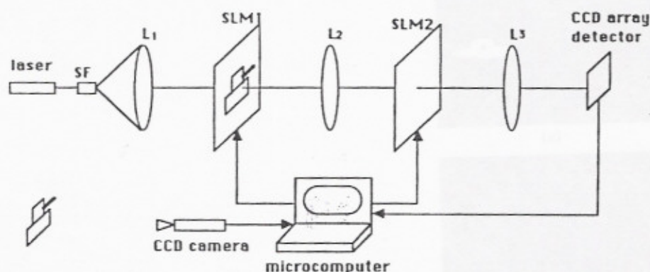
FIGURE 6.1 A microcomputer-based optical processor. Note: L_1 is the collimated lens and L_2 and L_3 represent the Fourier-transform lenses.
