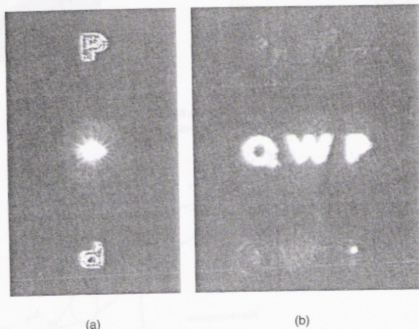
Figure 8.19 Photographs of (a) the impulse response of a VanderLugt filter, and (b) the response of the filter to the letters Q, W, and P.
