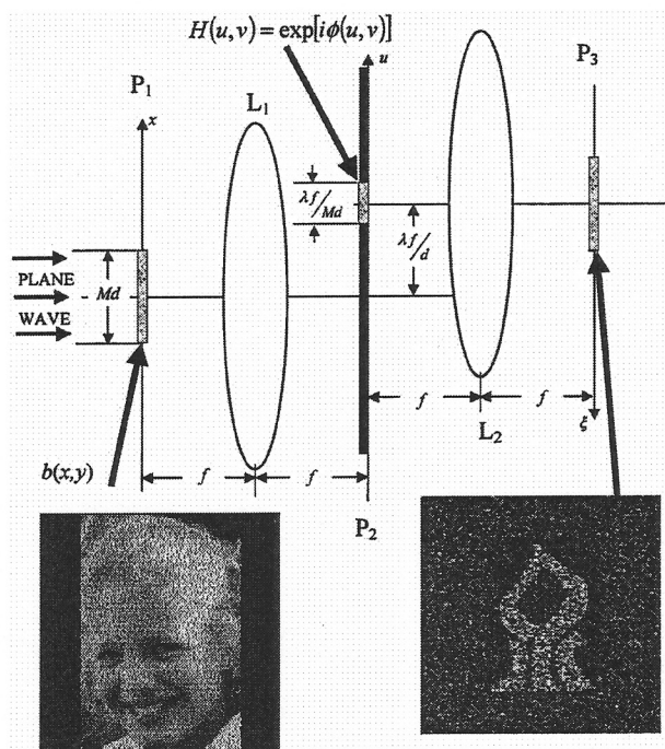
Fig. 4. Optical correlator that can be used to reveal the hidden image in the halftone picture.
