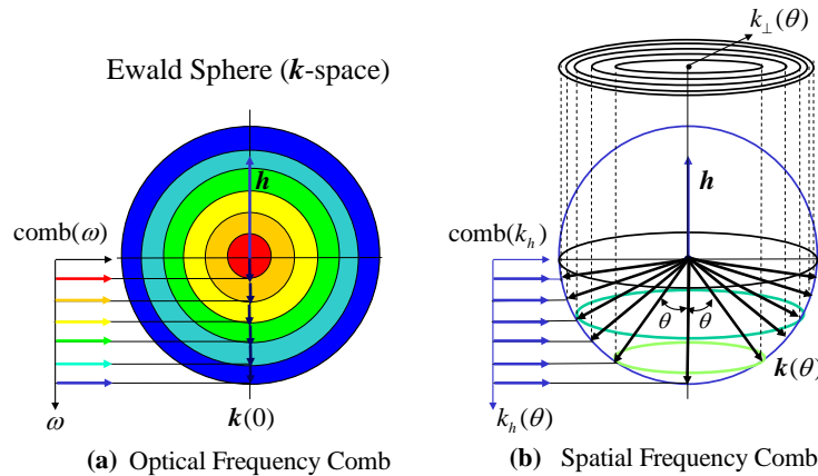
Fig.4 (a) Optical frequency comb is represented by collinear \mathbf{k} -vectors of different lengths for polychromatic light; (b) spatial frequency comb is represented by \mathbf{k} -vectors of the same length for monochromatic light but with different angles that give a polychromatic effect to the projected depth components of the \mathbf{k} -vectors.
